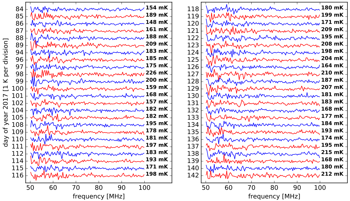
Figure 2: Daily residuals to 7-term polynomial over 50-100 MHz, for all days considered. The GHA range is 0-24 hr.
