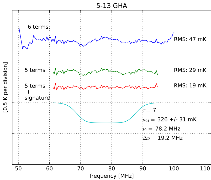
Figure 8: Residuals for average over 5-13 GHA, to 1) 6-term polynomial over 50-100 MHz (blue); 2) 5-term polynomial over 61-95 MHz (green); 3) 5-term polynomial plus 21-cm signature over 61-95 MHz (red). Also shown (cyan) is the best fit 21-cm signature over 61-95 MHz.
